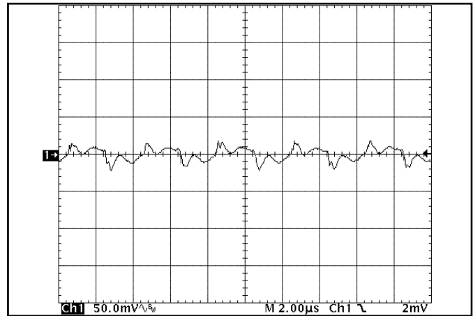
Figure 20: Output voltage ripple at nominal input voltage and rated load current (50 mV/div). Load capacitance: 1\ \mu\text{F} ceramic capacitor and 10\ \mu\text{F} tantalum capacitor. Bandwidth: 500 MHz. See Figure 17.
