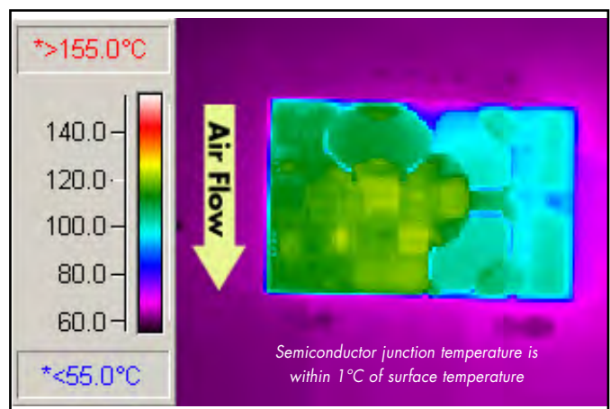
Figure 12: Thermal plot of converter at 45 amp load current with 55°C air flowing at the rate of 200 LFM. Air is flowing from pin 1 to pin 3 (nominal input voltage and 4 output pins).
