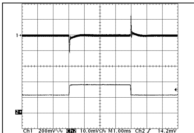
Figure 16: Output voltage response to step-change in load current (50%-75%-50% of I_{out(max)} ; dI/dt = 1A/\mu s ). Load cap: 470 \mu F , 30 m \Omega ESR tantalum capacitor and 1 \mu F ceramic cap. Ch 1: Vout (200mV/div), Ch 2: Iout (20A/div).
