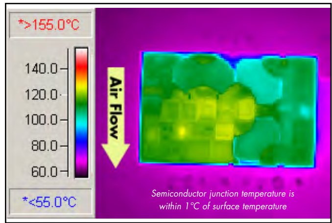
Figure 8: Thermal plot of converter at 41 amp load current with 55°C air flowing at the rate of 200 LFM. Air is flowing from pin 1 to pin 3 (nominal input voltage and 2 output pins).
