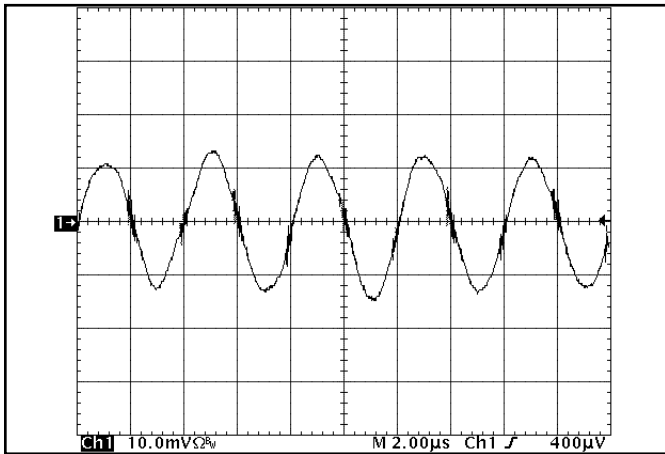
Figure 19: Input reflected ripple current, i_s , through a 10\ \mu\text{H} source inductor at nominal input voltage and rated load current (5 mA/div). See Figure 17.
