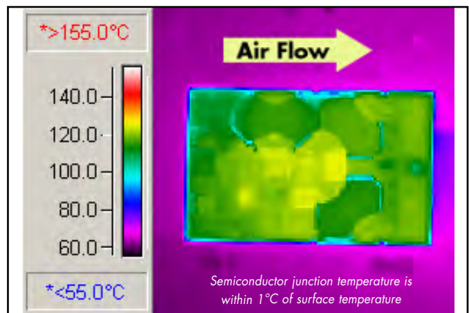
Figure 6: Thermal plot of converter at 41 amp load current with 55°C air flowing at the rate of 200 LFM. Air is flowing from input to output (nominal input voltage and 2 output pins).
