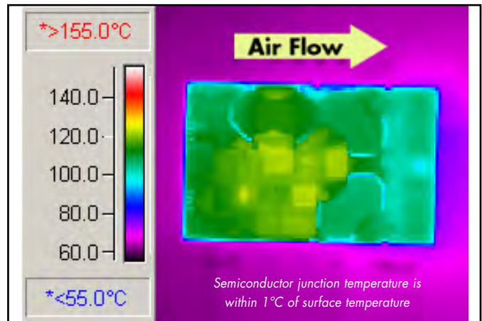
Figure 10: Thermal plot of converter at 45 amp load current with 55°C air flowing at the rate of 200 LFM. Air is flowing from input to output (nominal input voltage and 4 output pins).
